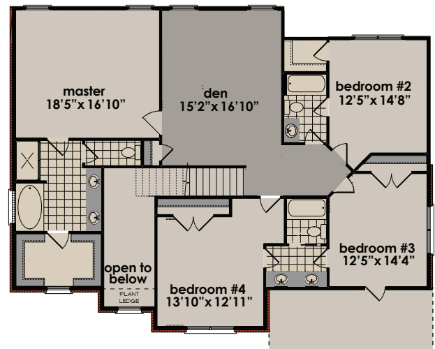
Upper Level Floor
