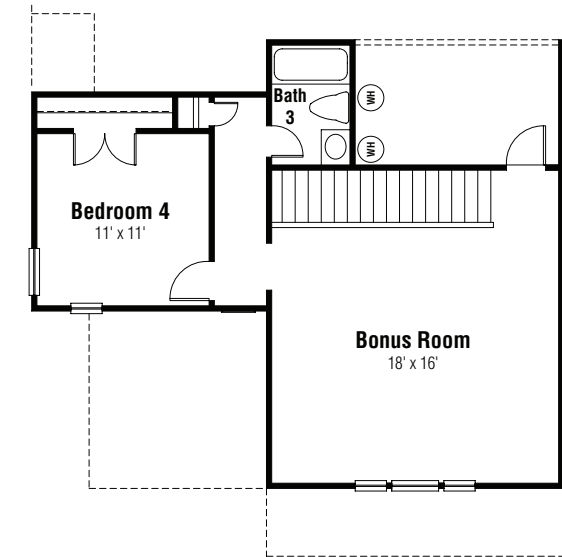
Optional Bonus Room w/ Bedroom 4
