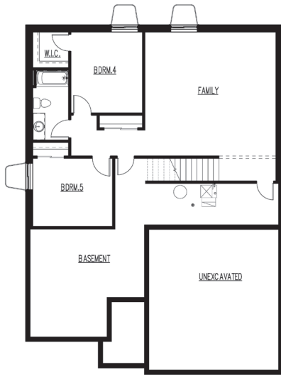
LOWER LEVEL
