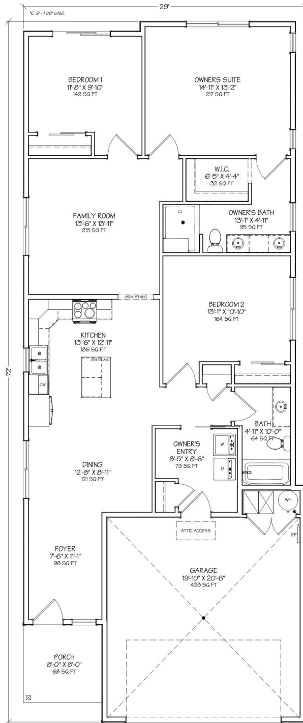
Roberta 2.0 - Base Plan - Main Floor - 1,487 sq ft
