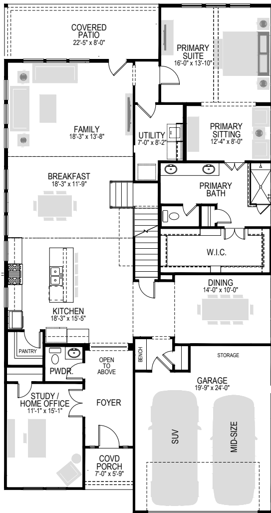
FIRST FLOOR
