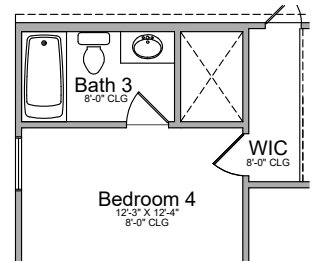
Opt. Bath 3 @ Bedroom 4
