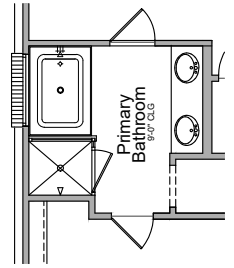
Opt. Primary Bath w/ Skirted Acrylic Tub
