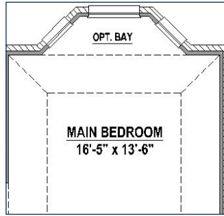
Main Bay Window (+27 SF)
