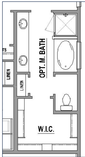
Optional Main Bath Layout
