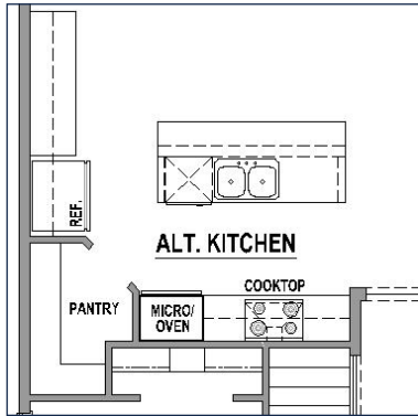
Alternate Kitchen Layout
