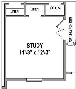
Optional French Doors at Study
