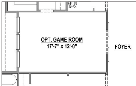
Optional Game Room
