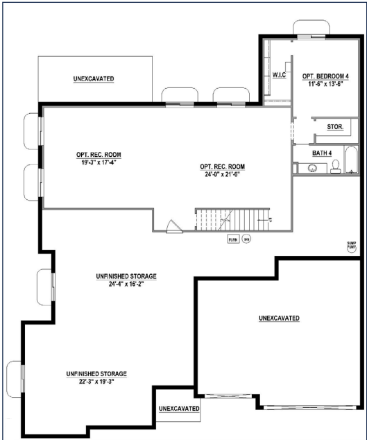
Optional Rec Room with Bedroom 4 and Bath 4 (+1,316 SF)
