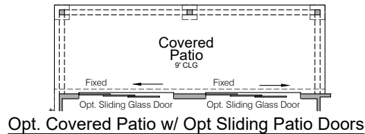
Second Floor
