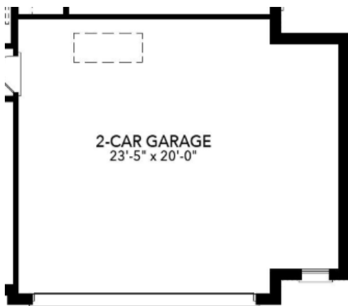
5ft Garage Extension
