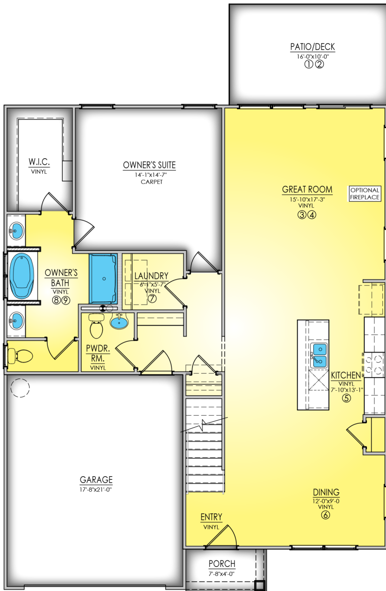
MAIN LEVEL - ELEVATION A
