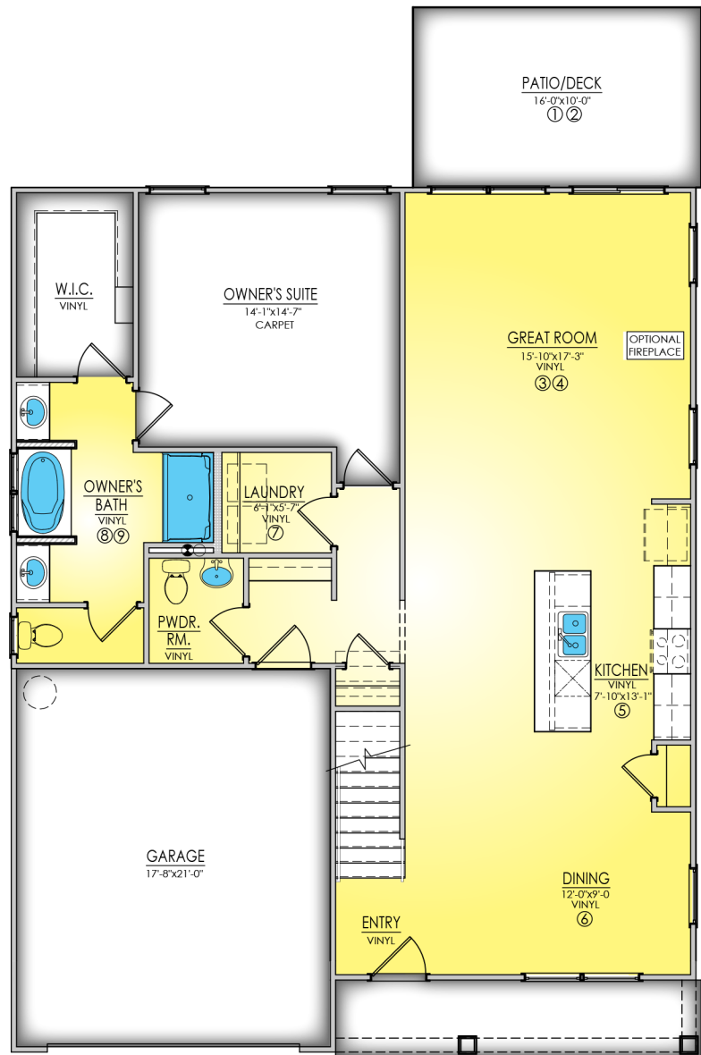
MAIN LEVEL - ELEVATION B
