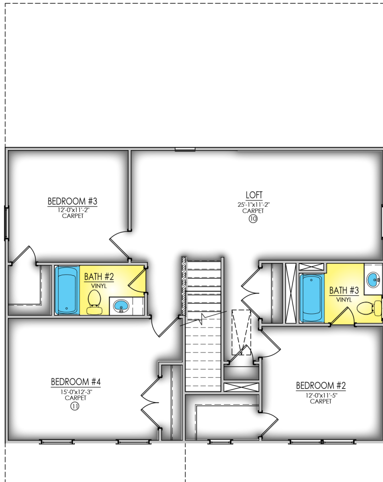
SECOND LEVEL - ELEVATION B
