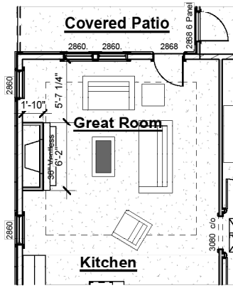
Great Room Fireplace Bump-In
