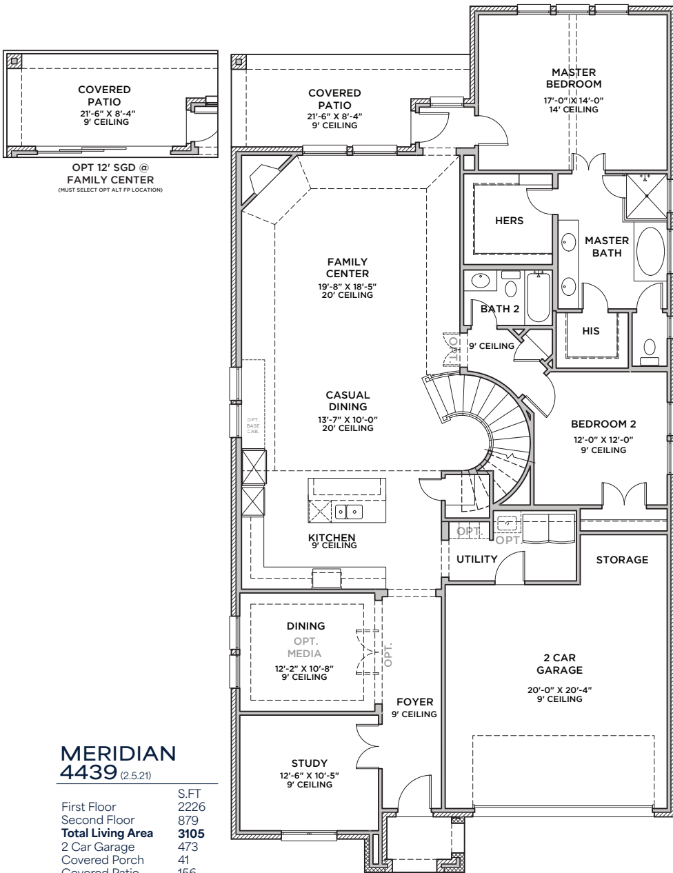
FIRST FLOOR
