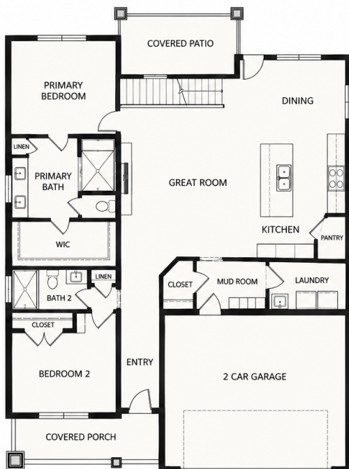
MAIN LEVEL 1,628 SQ. FT.
