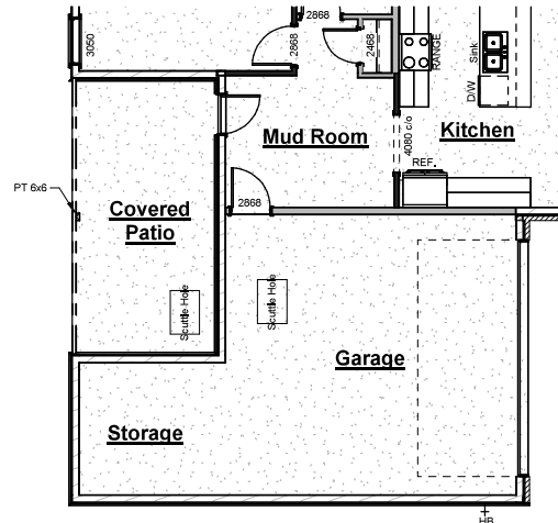
2-Car Garage with Storage
