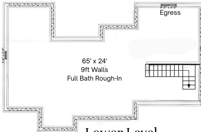
Lower Level
