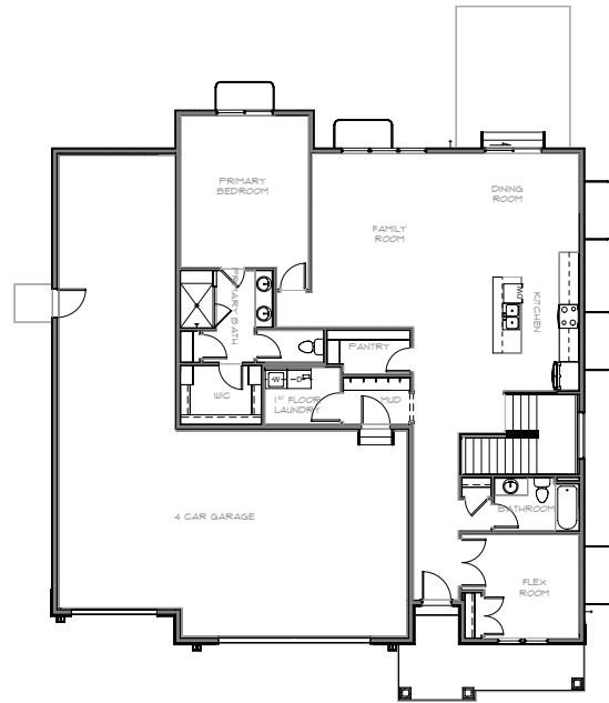
Main Floor
