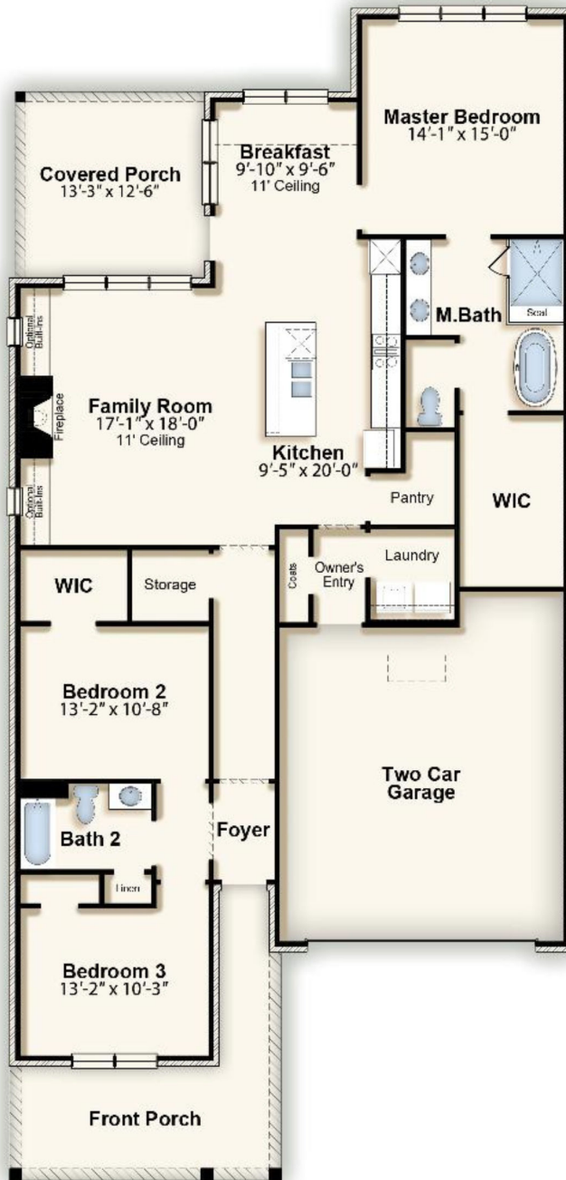
FIRST FLOOR - ELEV A
