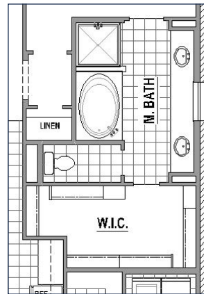
Optional Drop In Tub in Main Bath
