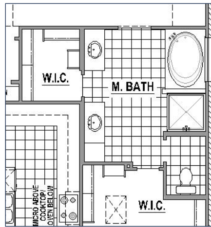
Optional Drop in Tub in Main Bath
