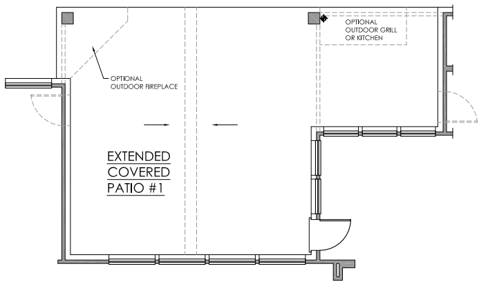
EXT'D COVERED PATIO #1 OPTION
