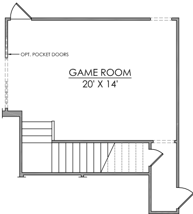
FIRST FLOOR WITH ALL BONUS OPTIONS
