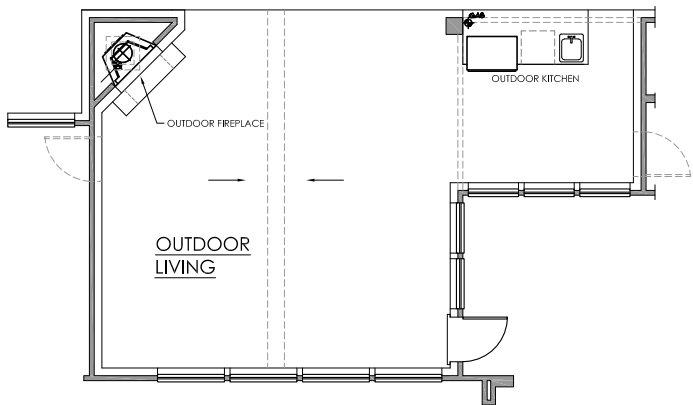
OUTDOOR LIVING OPTION
