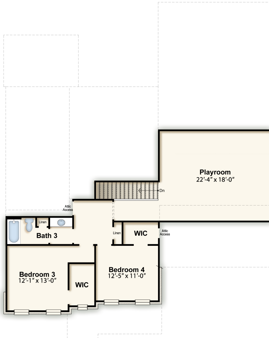
SECOND FLOOR - ELEV A
