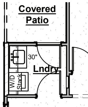
Laundry Room Sink Option
