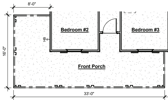
Wrap Around Front Porch
