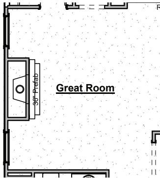
Great Room Fireplace Bump-In
