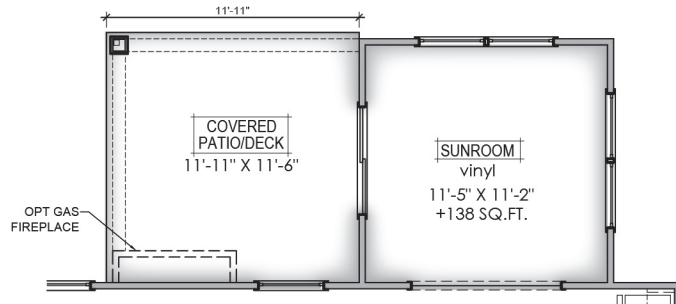
OPT SUNROOM W/ COVERED PATIO/DECK
