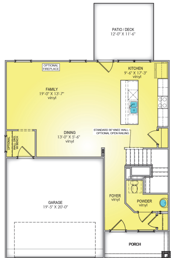
MAIN LEVEL PLAN - B
