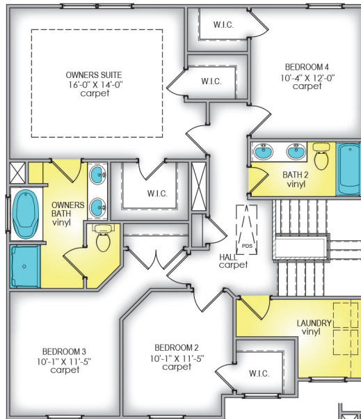
SECOND LEVEL PLAN - A
