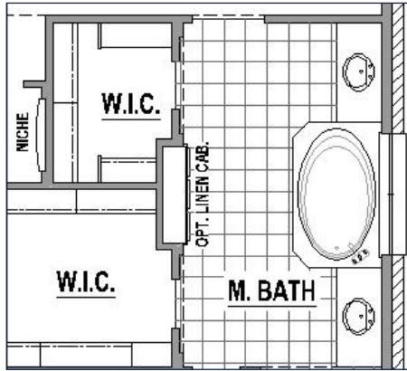
Linen Cabinet at Main Bath
