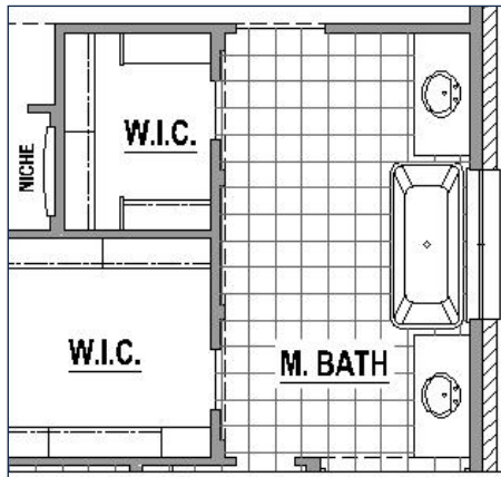
Freestanding Tub at Main Bath
