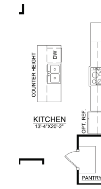
OPTIONAL PRESTIGE KITCHEN #1
