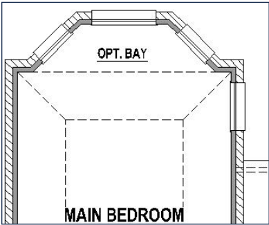
Main Bay Window (+27 SF)
