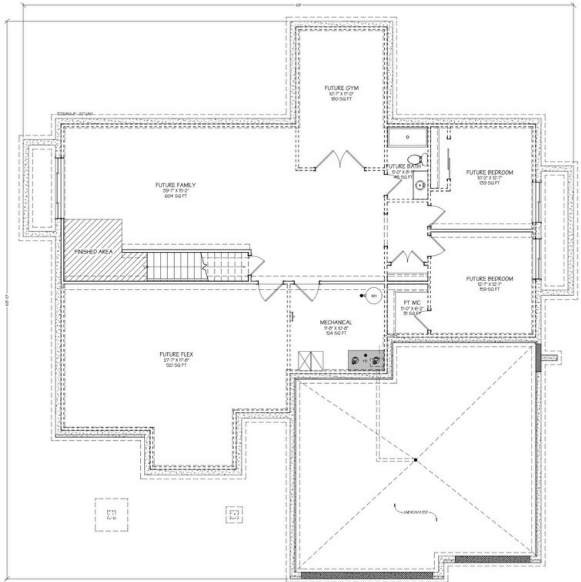
Valhalla 3.0 - Base Plan - Lower Floor - 2,275 sq ft
