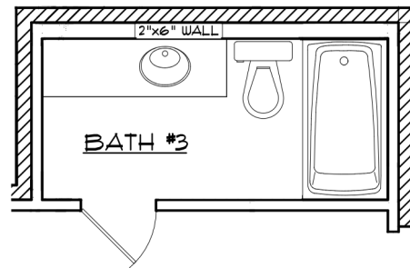
Opt. Bath 3 at Bedroom 4
