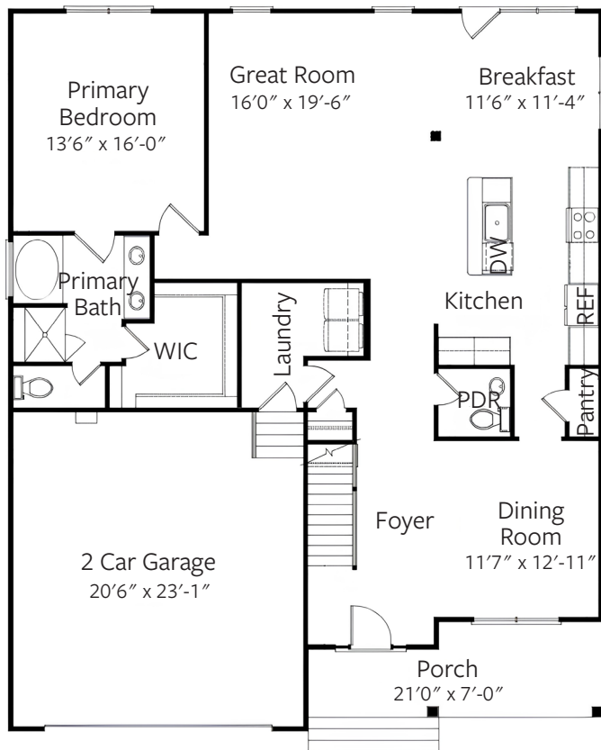
Included First Floor
