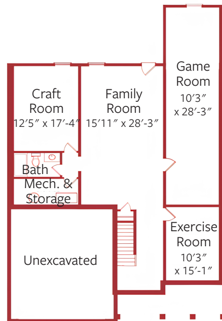
Optional Finished Basement with Optional Finished Craft Room, Optional Finished Family Room, Optional Finished Game Room, Optional Finished Bath, and Optional Finished Exercise Room
