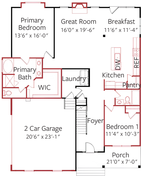
Included First Floor shown with Optional:
