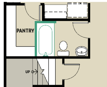
OPTIONAL FULL BATHROOM IN PLACE OF POWDER
