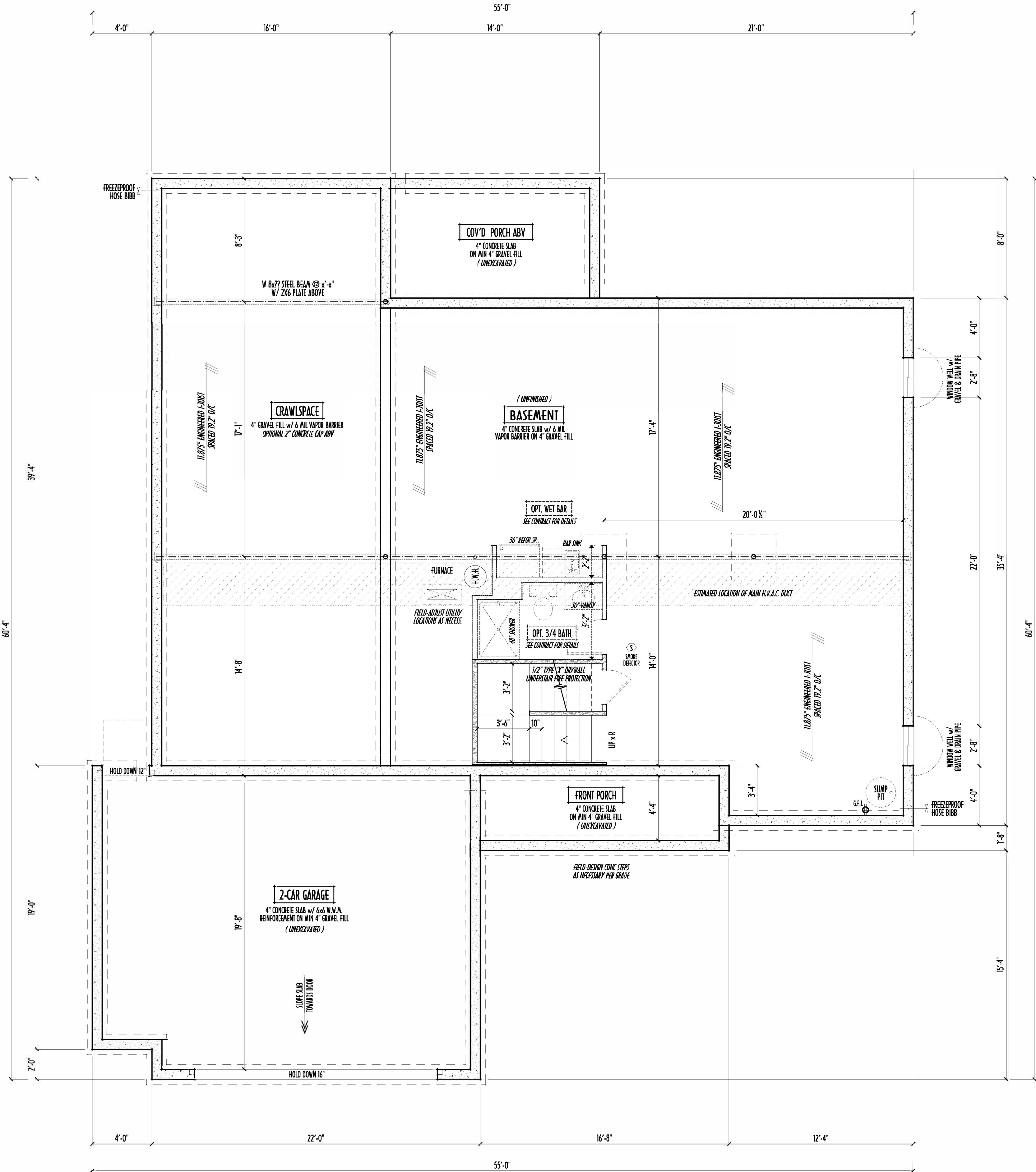
FOUNDATION / BASEMENT PLAN SCALE: 1/4" = 1'-0"
