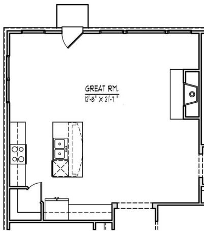
OPTIONAL FIREPLACE FIRST FLOOR PLAN
