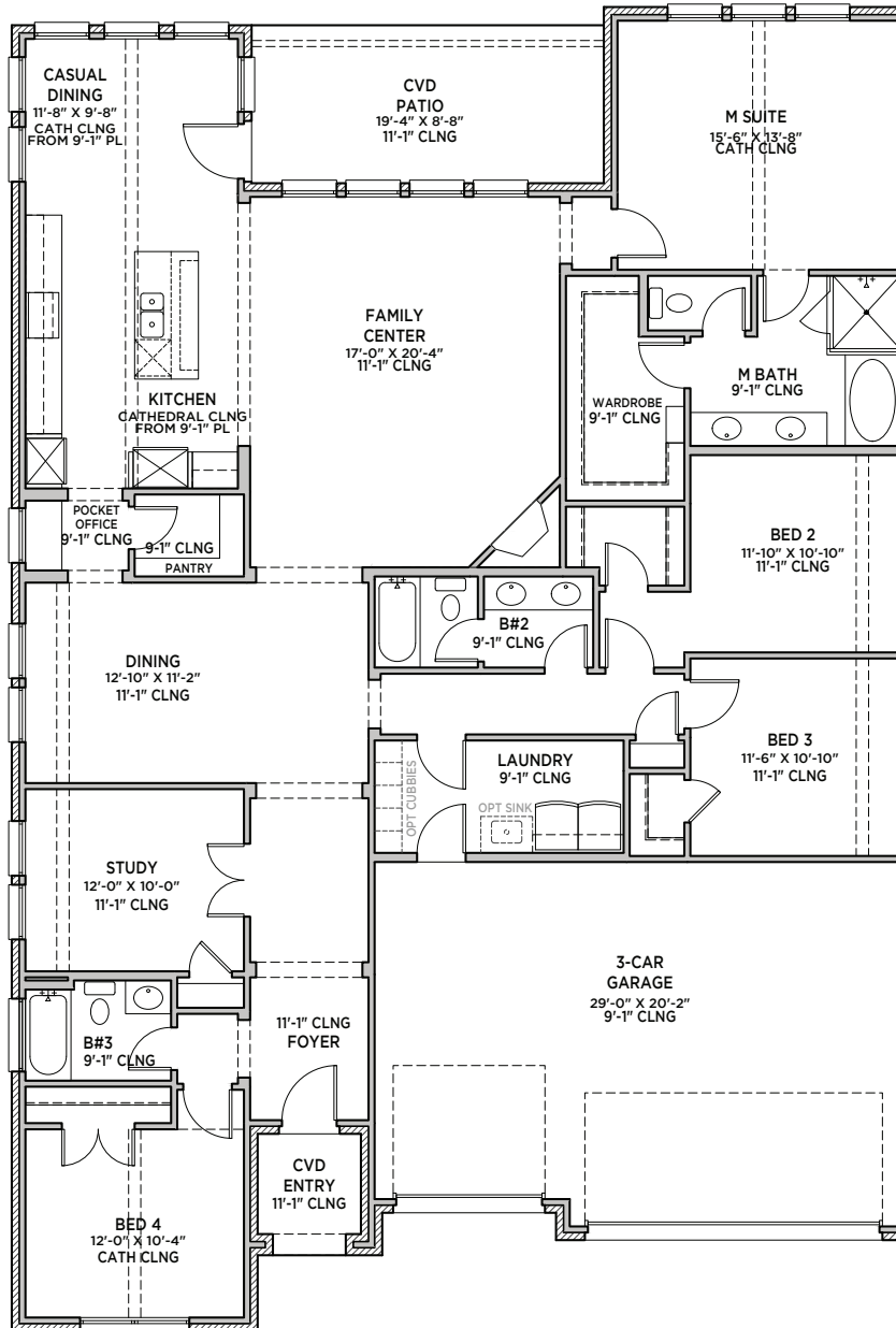
FIRST FLOOR
