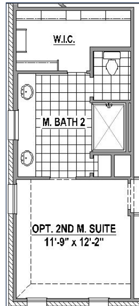
Optional 2nd Main Suite (+132 SF)
