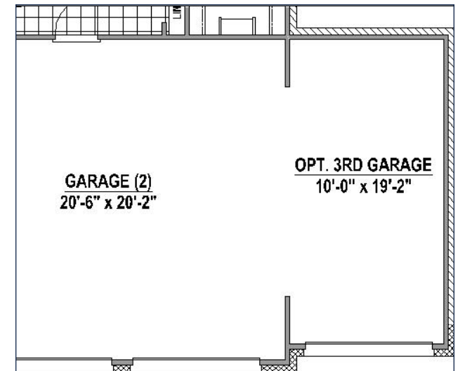
Optional 3rd Car Garage
