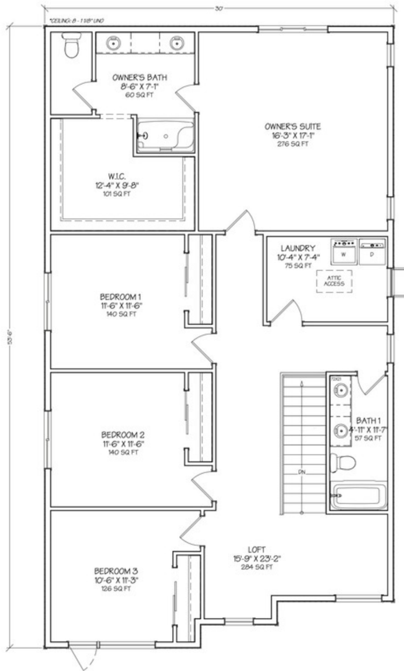
Arcadia 2.0 - Base Plan - Upper Floor - 1,562 sq ft
