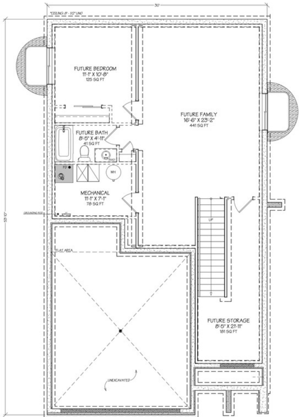
Arcadia 2.0 - Base Plan - Lower Floor - 1,073 sq ft
