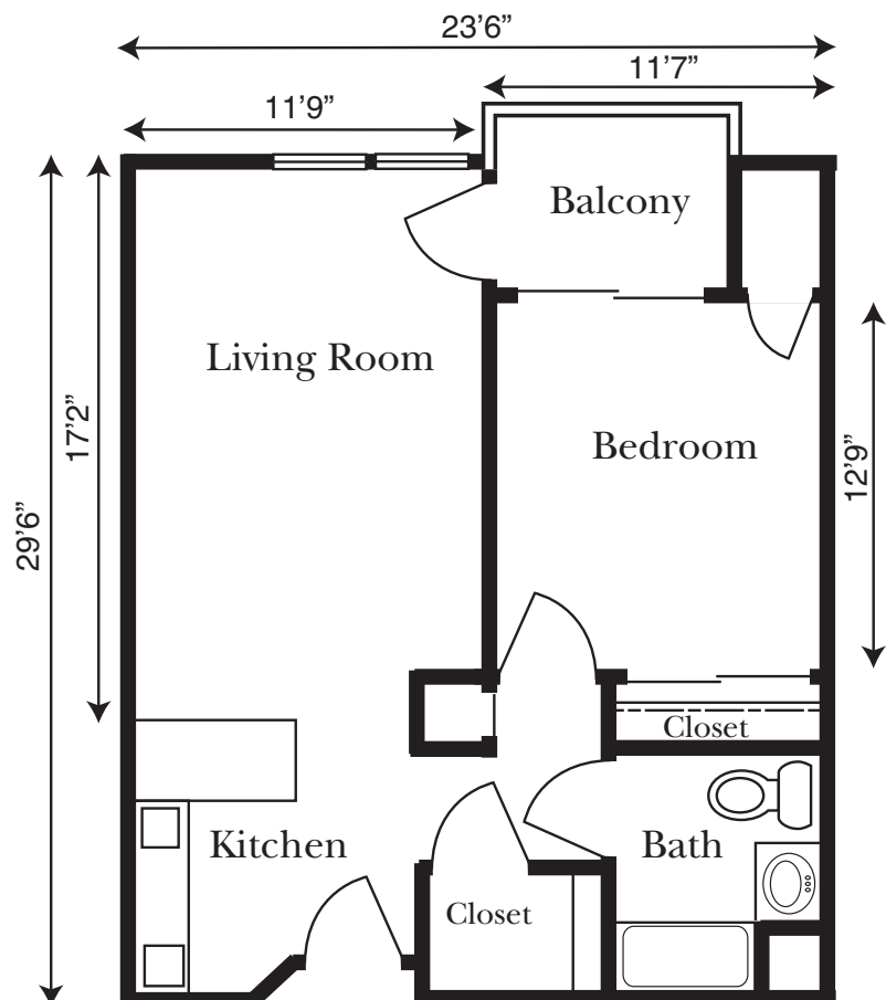
ONE BEDROOM 678 SQ. FT.
