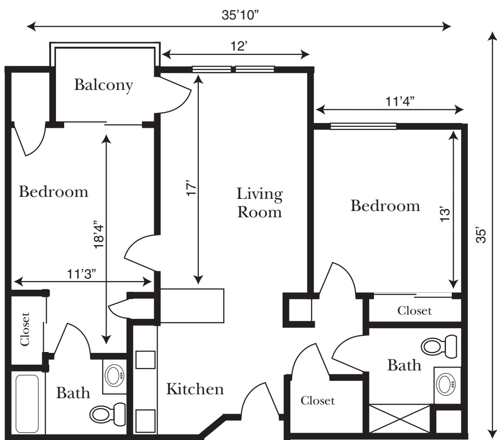
TWO BEDROOM, TWO BATH 973 SQ. FT.
