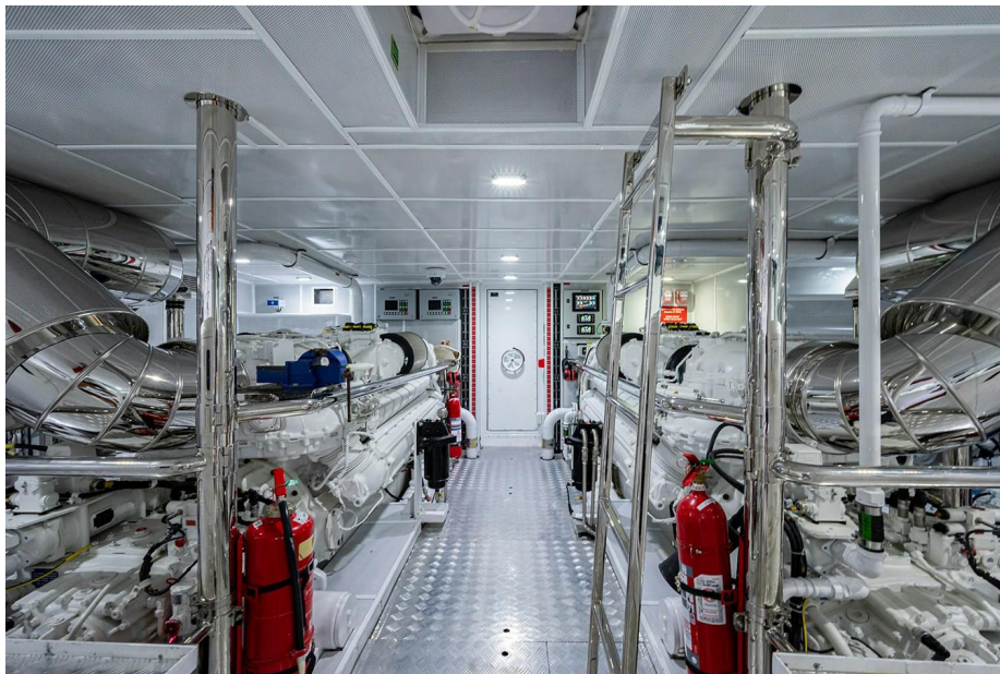
Engine Room
