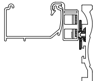
Bottom position
