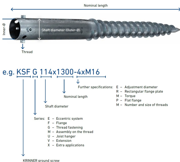
Fig. 1: All Krinner ground screws are made entirely of steel and are hot-dip galvanised.
