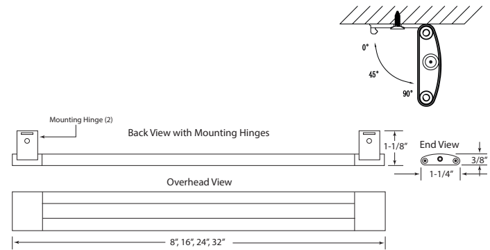
Above: LARC6 Fixture. Right: LARC6 with Rigid Inline Power Switch (LARC6-MS-W) Far Right: LARC6 with Rigid Inline Touch Dimmer (LARC6-TD-W) (Sold individually).
