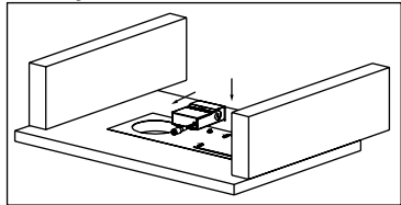
Figure 4: connect the electrical supply connection in the detachable junction box. Secure the junction box by placing it through the keyhole slot and attach luminaire using the connector.
