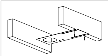
Figure 1: Nail-in the mounting plate to the ceiling joist (adjust plate as needed).
