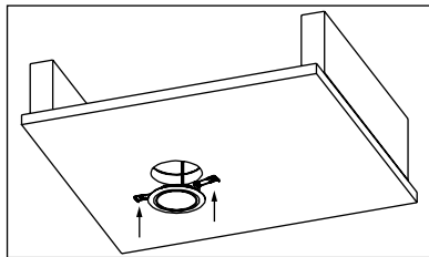
Figure 5: Push the spring clips up and through the hole of the ceiling. Release the spring clips and align luminaire to sit properly over the ceiling hole.
