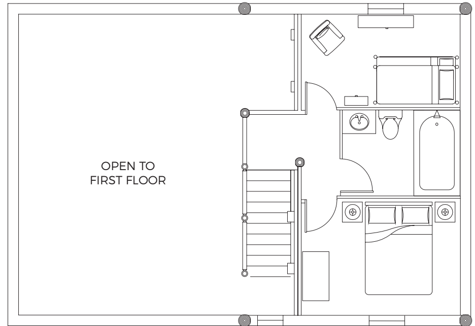
SECOND FLOOR
