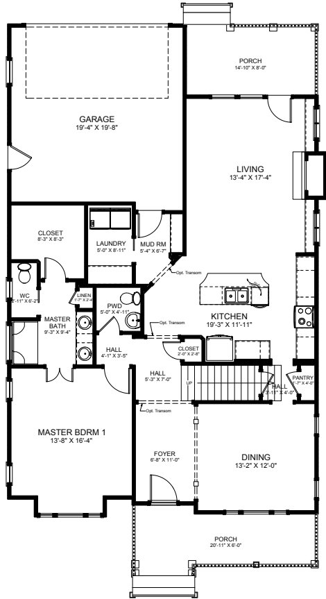
first floor A
