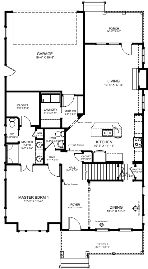
first floor B
