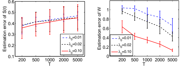
Figure 2. Estimation error of latent sources and factor loadings with different observation lengths and base rates
