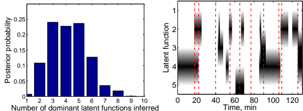
Figure 7. Posterior over number of dominant sources with a sample of sources (black represents 1 and red dash-dot lines delineate scenes the users were asked to recall)
