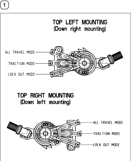
remote lever
