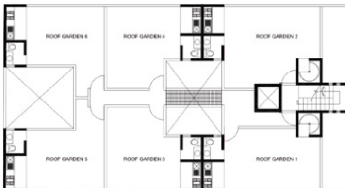
ROOF GARDEN
