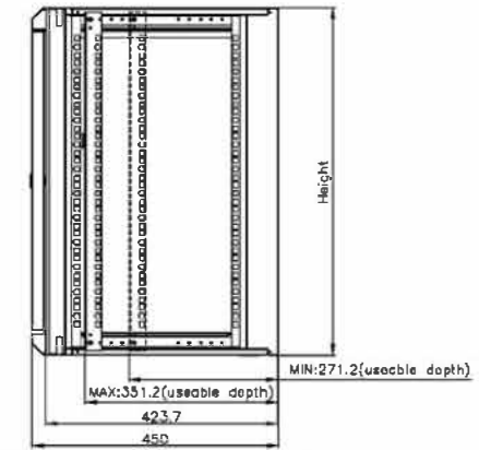
450 mm Depth
