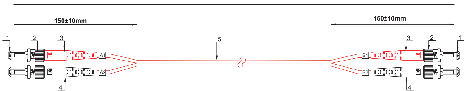
Cable Profile View
